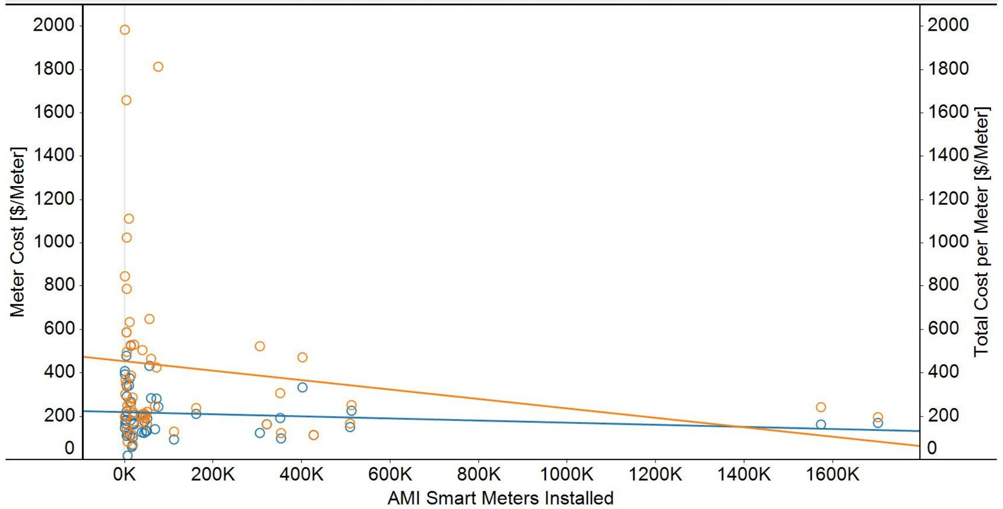
Meter Costs vs Number of Meters Installed per Project
