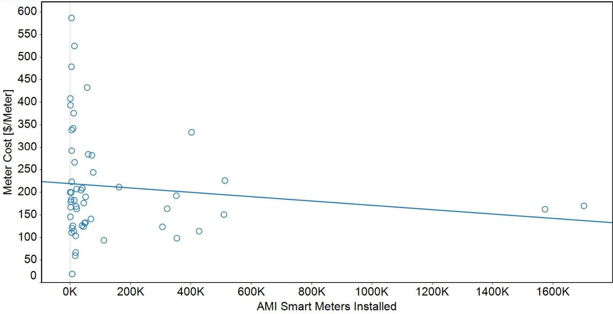
Meter Cost vs. Number of Meters Installed per Project
