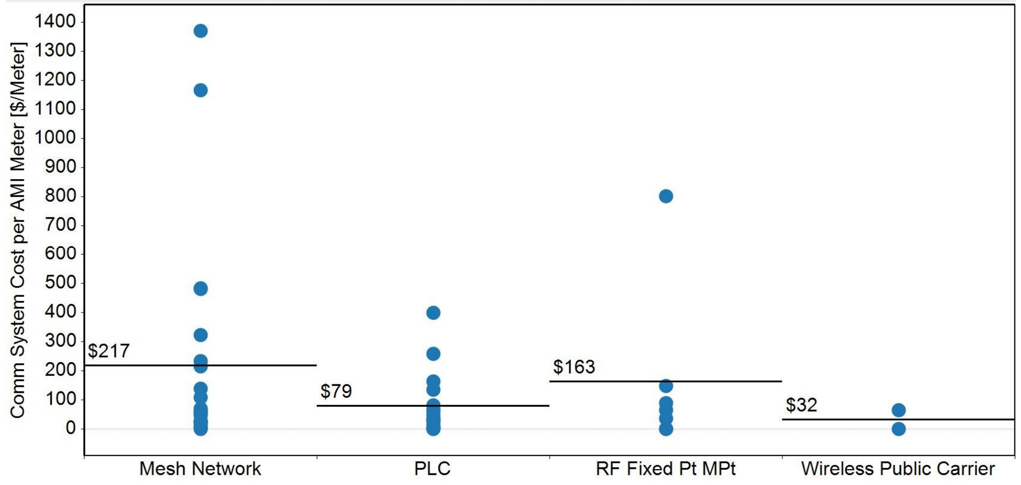
Communication System Costs by Project and System Type
