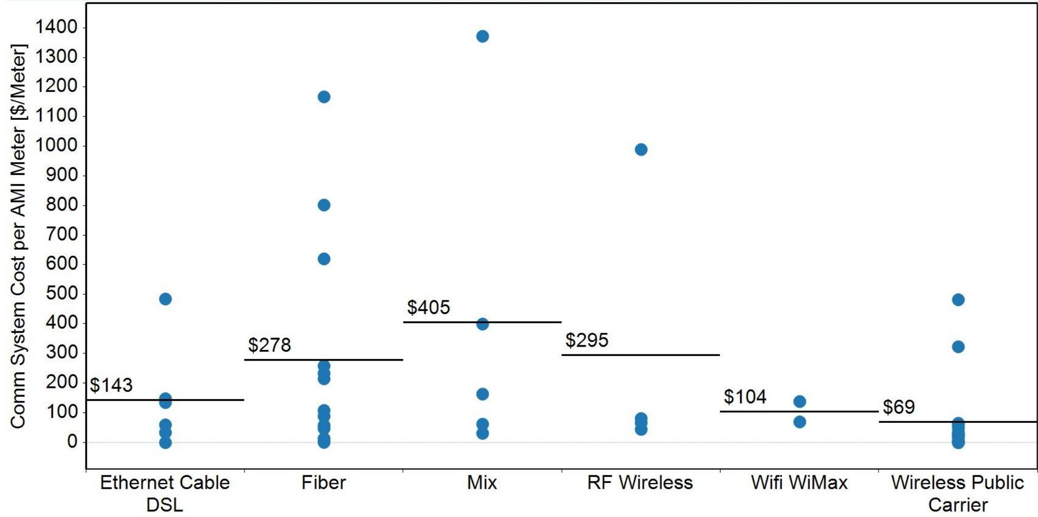
Communication System Costs by Project and Backhaul Network Type
